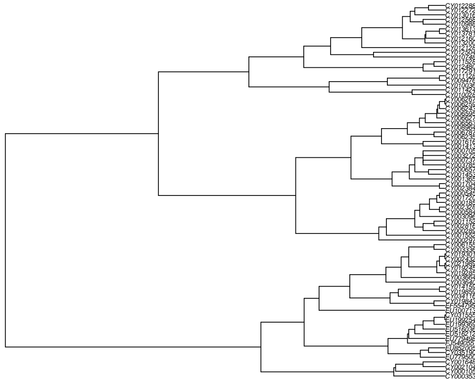
UPGMA tree
